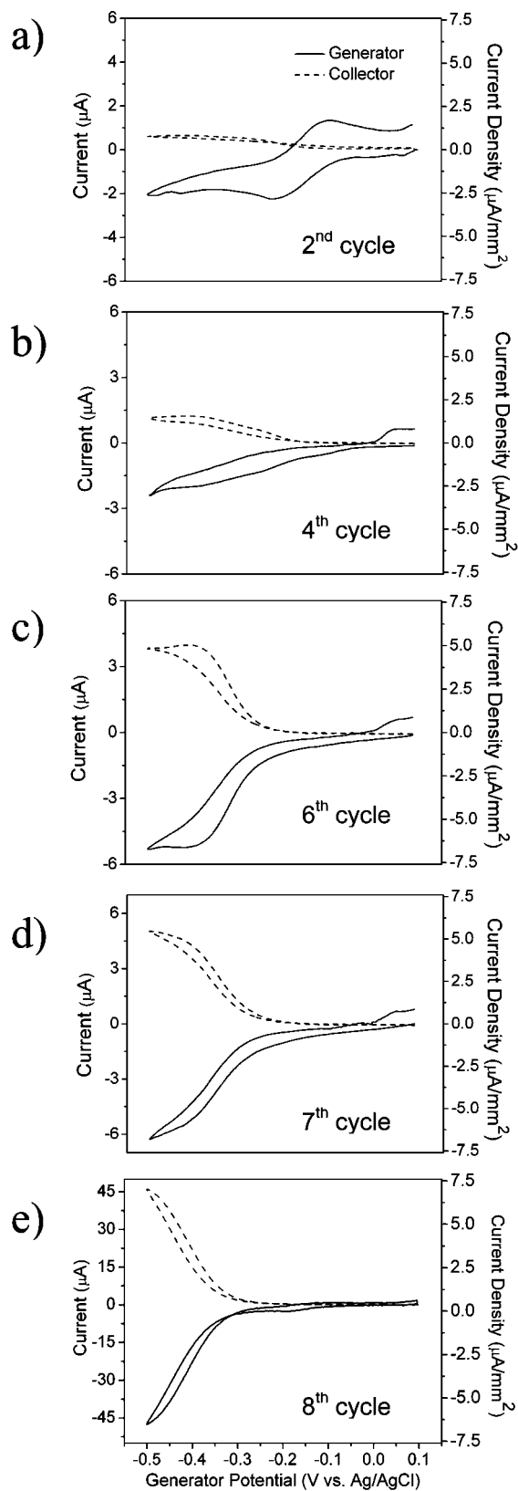
Figure 4. Generation-collection voltammograms of 1 mM \text{Ru}(\text{NH}_3)_6^{3+} in a \text{Hg}-\text{SC}_{10}\text{COO}^-//\text{Ru}(\text{NH}_3)_6^{3+2+}//-\text{OOC}_{10}\text{S}-\text{Hg} junction in 0.1 M NaF at pH 9. The collector potential was held at +0.10 V, and the generator potential was cycled between +0.10 and -0.50 V at a scan rate of 50 mV/s (solid line, generator current; dashed line, collector current). The area of the junction was ca. 0.79 \text{mm}^2 throughout this set of experiments.
